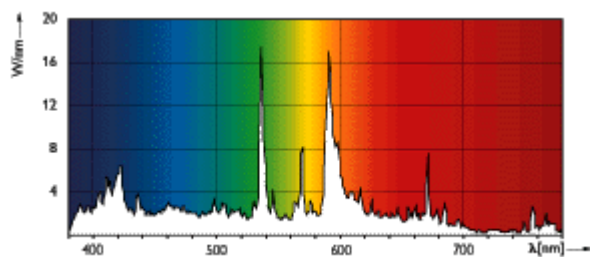
MASTER MHN-SA 2000W /956
