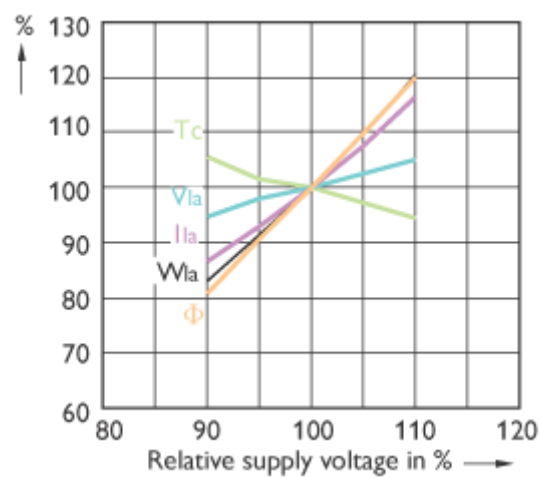
MASTER MHN-SA 2000W 400V
