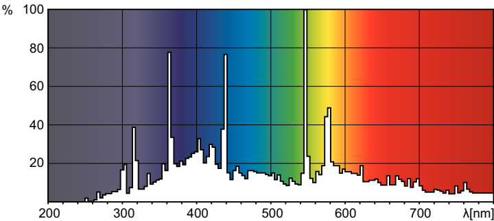
Spectral Power Distribution Colour - MSD Gold 300/2 MiniFastFit 1CT/16
