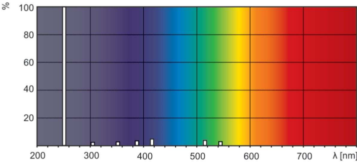
Spectral Power Distribution Colour - TUV 16W IN FAM/10X25BOX
