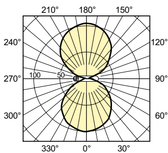
Light Distribution Diagram - MST SON-T PIA Plus 400W E E40 1SL/12
